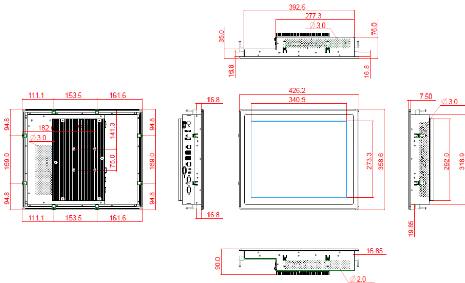
WLP-7F20-17 Outline Drawing (Panel Mount)
