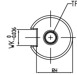
SHAFT END DETAILS
